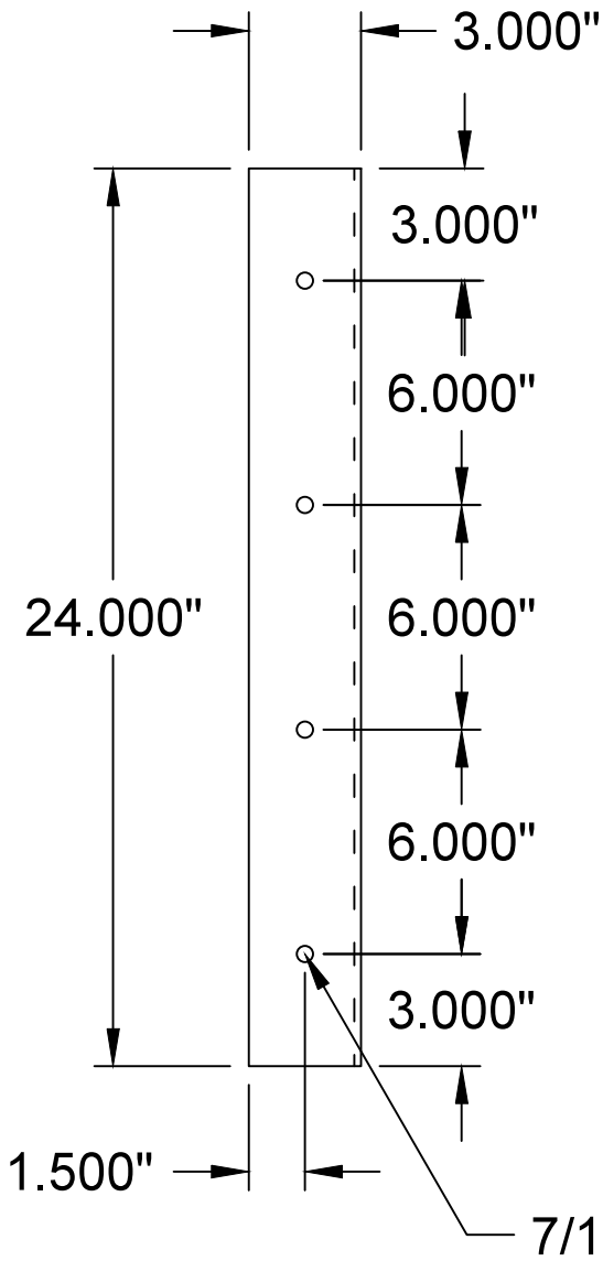
END VIEW
