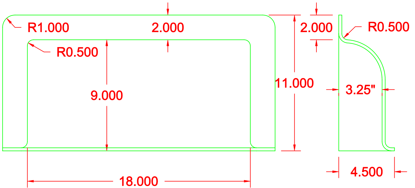
PLAN VIEW
