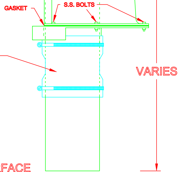
ASSEMBLY VIEW (WITH SNOUT ATTACHED)
