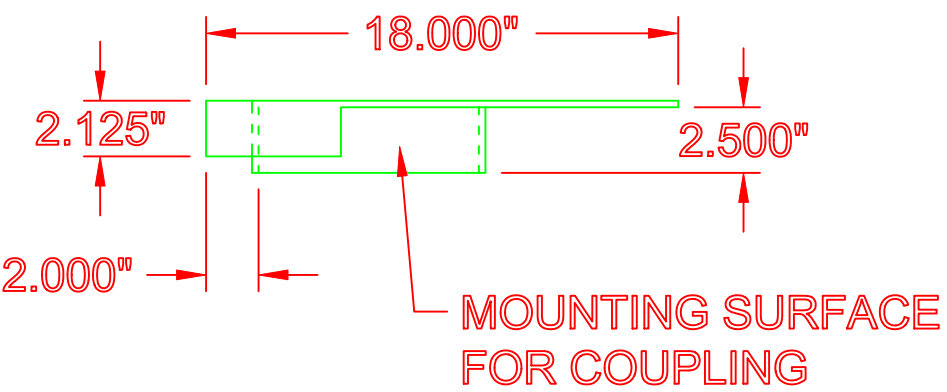
SIDE (RESTRICTOR PLATE ONLY)
